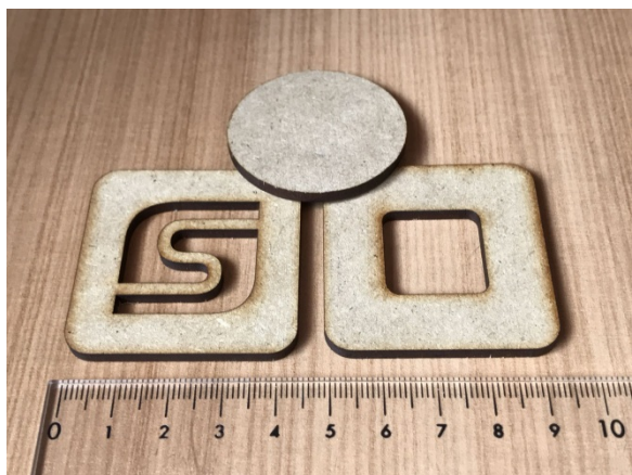
13 - MDF 3 mm, F 9 mm/s, Pwr 255
